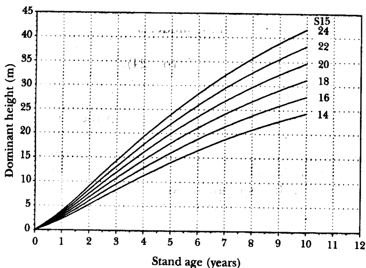
Figure 1. Dominant height growth curves for different site indices (eq. 3)
