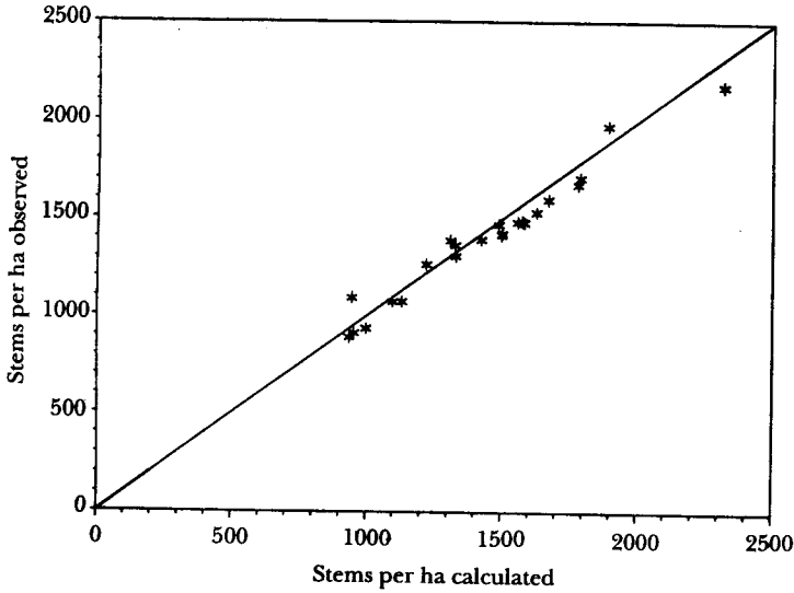
Figure 2. Comparison of observed and calculated survivals (eq. 4)
