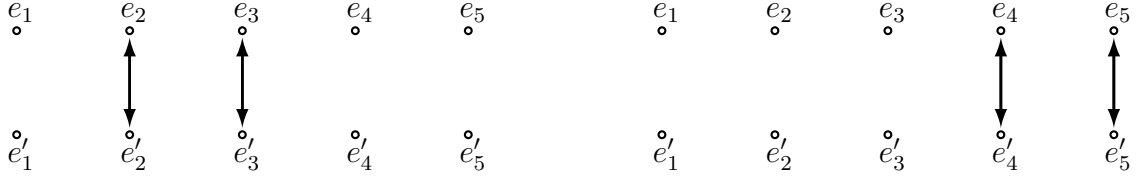
FIGURE 8. Further generators that yield H^1(G, \mathfrak{P}) = \mathbb{Z}/4\mathbb{Z} \oplus \mathbb{Z}/2\mathbb{Z}
