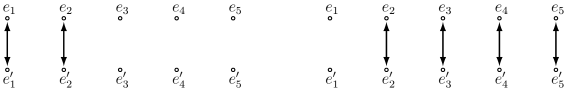
FIGURE 3. Generators of the order 4 group
