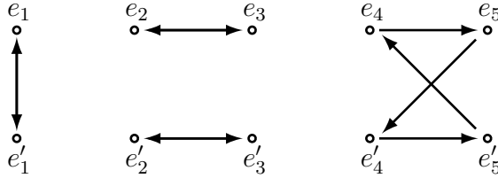
FIGURE 5. The generator of the cyclic group G of order 4
