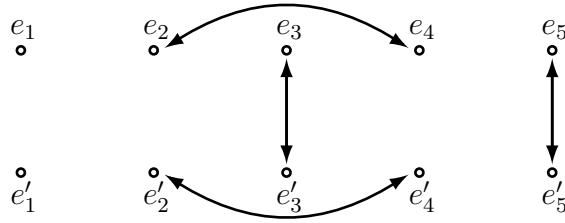
FIGURE 11. The operation of the decomposition group at infinity
