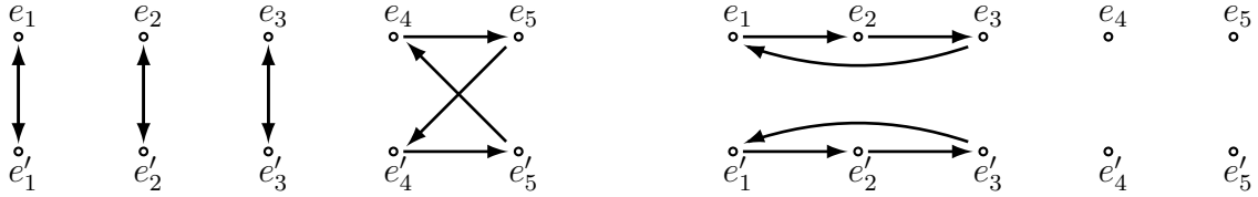
FIGURE 4. The element \tau and one of the possible elements \sigma \in S_3
