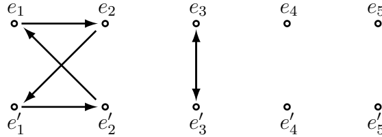
FIGURE 2. The generator of the cyclic group G
