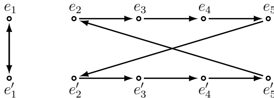
FIGURE 6. The generator of the cyclic group G of order 8
