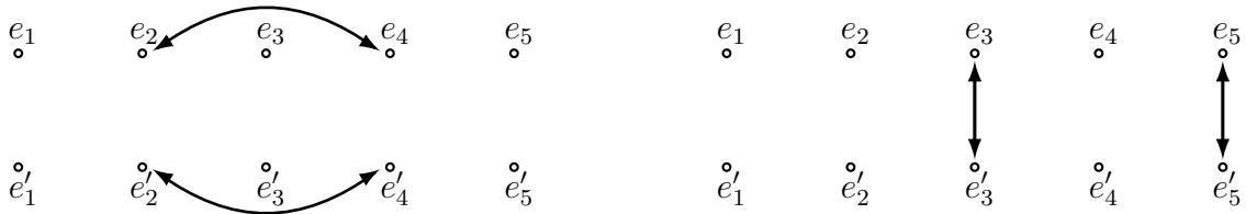
FIGURE 12. Generators of the decomposition group at p = 19
