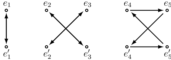
FIGURE 7. A generator of a cyclic group of order 4
