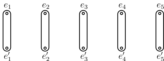
FIGURE 1. The combinatorial structure of the ten linear systems of conics
