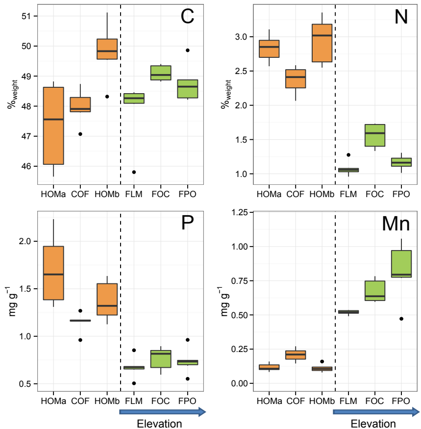
Figure 3. Contents of selected elements (C, N, P, Mn) in leaf litter from six ecosystems at Mt. Kilimanjaro. Medians, interquartile distances and extreme values are displayed as bold lines, boxes with whiskers and dots, respectively. Managed (left) and natural (right) ecosystems are separated by dashed line.
